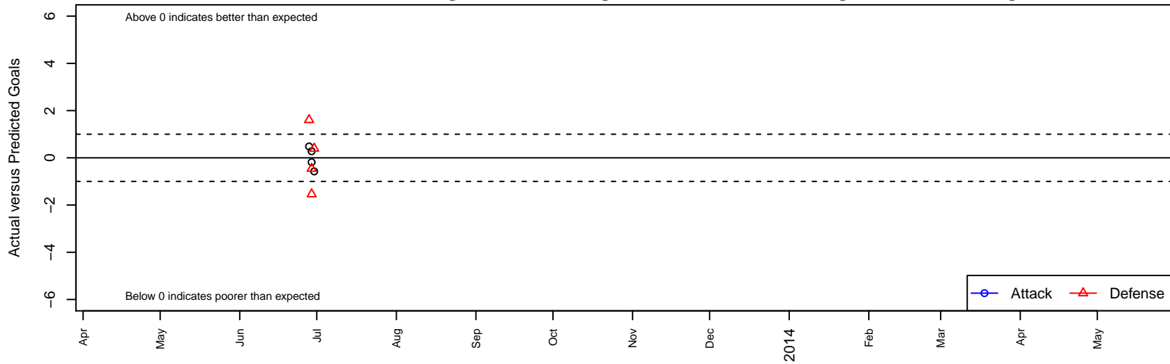
Columbia United Hermiston Heat –Unk B97 Dots are actual minus expected GF (blue circles) and GA (red triangles). Blue line is smoothed change in attack strength. Red is smoothed change in defense strength.
